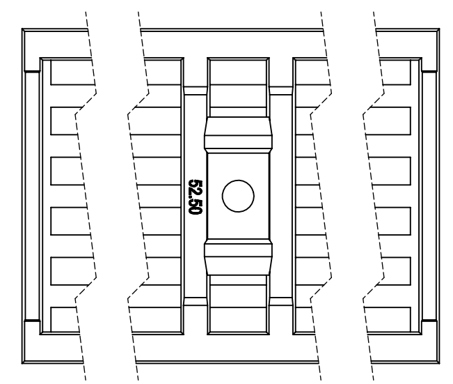
VIEW G
